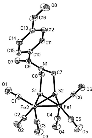
Figure 4. Molecular structure of 7 with 30% probability level ellipsoids.
