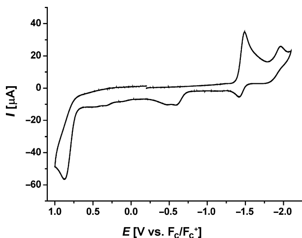
Figure 5. Cyclic voltammogram of 2 (1.0 mM) in 0.1 M n Bu 4 NPF 6 /MeCN at a scan rate of 100 mV s –1 .
