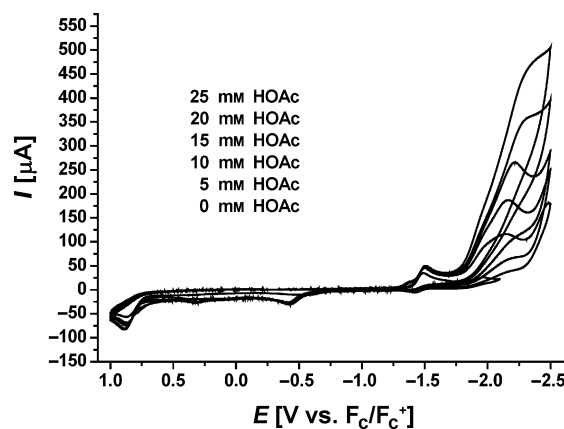
Figure 6. Cyclic voltammogram of 2 (1.0 mM) with HOAc (0–25 mM) in 0.1 M n Bu 4 NPF 6 /MeCN at a scan rate of 100 mV s –1 .
