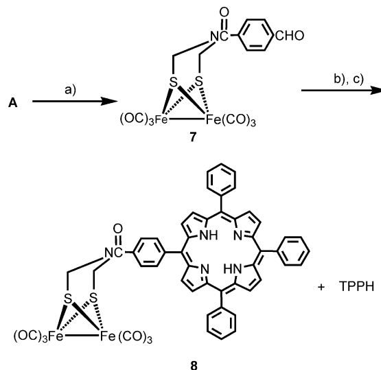
Scheme 3. (a) p - \text{CHOC}_6\text{H}_4\text{C(O)Cl} , \text{Et}_3\text{N} , \text{CH}_2\text{Cl}_2 , 0 °C to room temp.; (b) \text{PhCHO} , pyrrole, \text{BF}_3\cdot\text{Et}_2\text{O} , \text{CH}_2\text{Cl}_2 , room temp.; (c) p -chloranil, \text{CH}_2\text{Cl}_2 , reflux.
