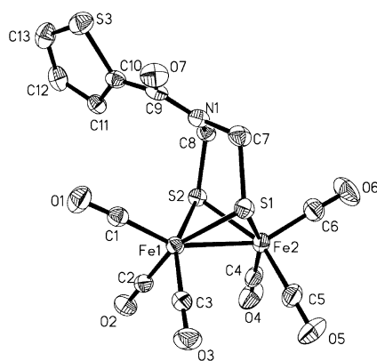
Figure 3. Molecular structure of 5 with 30% probability level ellipsoids.
