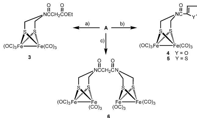
Scheme 2. (a) \text{EtO}_2\text{CCH}_2\text{C(O)Cl} , pyridine, \text{CH}_2\text{Cl}_2 , 0^\circ\text{C} to room temp.; (b) \text{C}_4\text{H}_3\text{YC(O)Cl} , \text{Et}_3\text{N} , \text{CH}_2\text{Cl}_2 , room temp.; (c) \text{ClC(O)CH}_2\text{C(O)Cl} , pyridine, \text{CH}_2\text{Cl}_2 , 0^\circ\text{C} to room temp.
