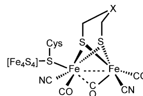
Figure 1. Basic structure of the H-cluster ( \text{X} = \text{CH}_2 , \text{NH} , or \text{O} ).
