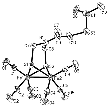
Figure 2. Molecular structure of 2 with 30% probability level ellipsoids.
