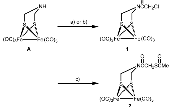
Scheme 1. (a) \text{ClCH}_2\text{CO}_2\text{H} , DCC, \text{CH}_2\text{Cl}_2 , 0^\circ\text{C} to room temp.; (b) \text{ClCH}_2\text{C(O)Cl} , \text{Et}_3\text{N} , THF, 0^\circ\text{C} to room temp.; (c) \text{MeC(O)SK} , THF, MeOH, 0^\circ\text{C} to room temp.
