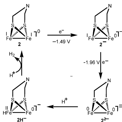
Scheme 4. Proposed 2E2C mechanism for H 2 evolution catalyzed by 2 . All terminal carbonyl groups and the N-functionalities are omitted for clarity.
